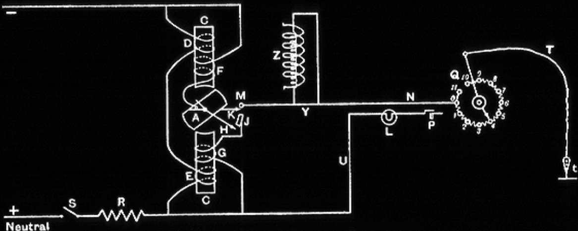
DIAGRAM OF CONNECTIONS OF AN OSCILLOCLAST.
