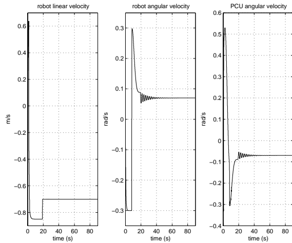
Fig. 4. The Follower Velocities and the PCU Velocity.
