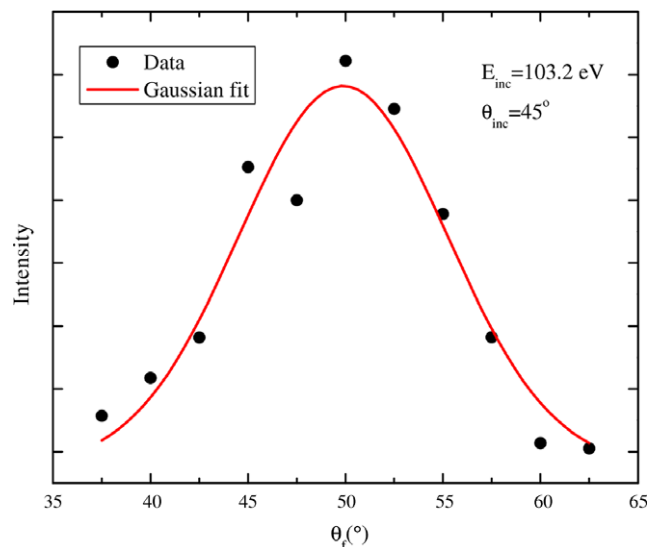
Fig. 4. An angular intensity spectrum obtained for Cs + ions scattered from Ag(001) along the \langle 110 \rangle azimuth at an incident angle of 45°. This spectrum was produced by integrating individual ESA spectra across a range of final scattered angles.
