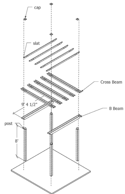
06 ISO-EXPLODED
