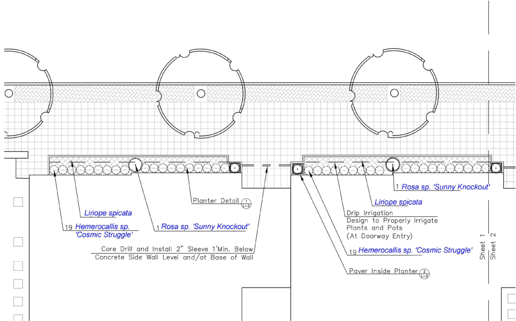
Landscape Plan: Sheet 1 Scale: 1" = 10'-0"
