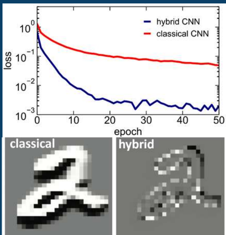
Training loss and feature selection for classical and hybrid quantum-classical convolutional neural networks
