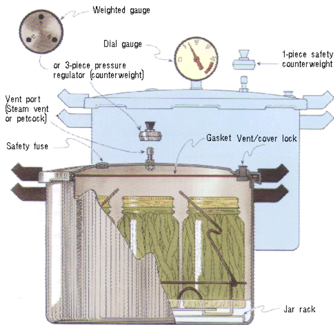
Figure 2. Pressure Canner
