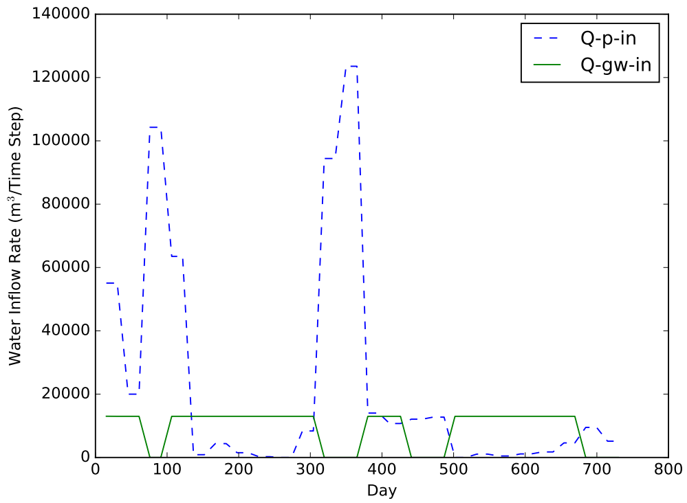
Figure 6: Volumetric water usage from wells and rainfall events over the two year horizon
