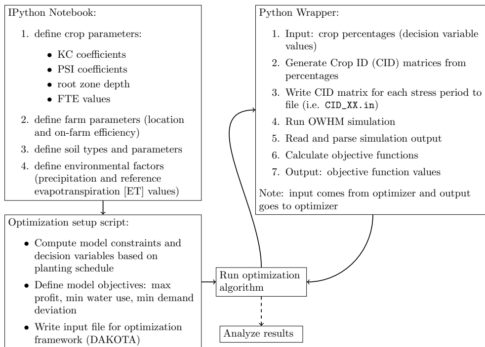
Figure 1: An interactive IPython notebook is used as a preprocessing step to generate data files and define the optimization problem. Then a set of python wrappers executes the communication between the simulation tool and the optimization algorithm.
